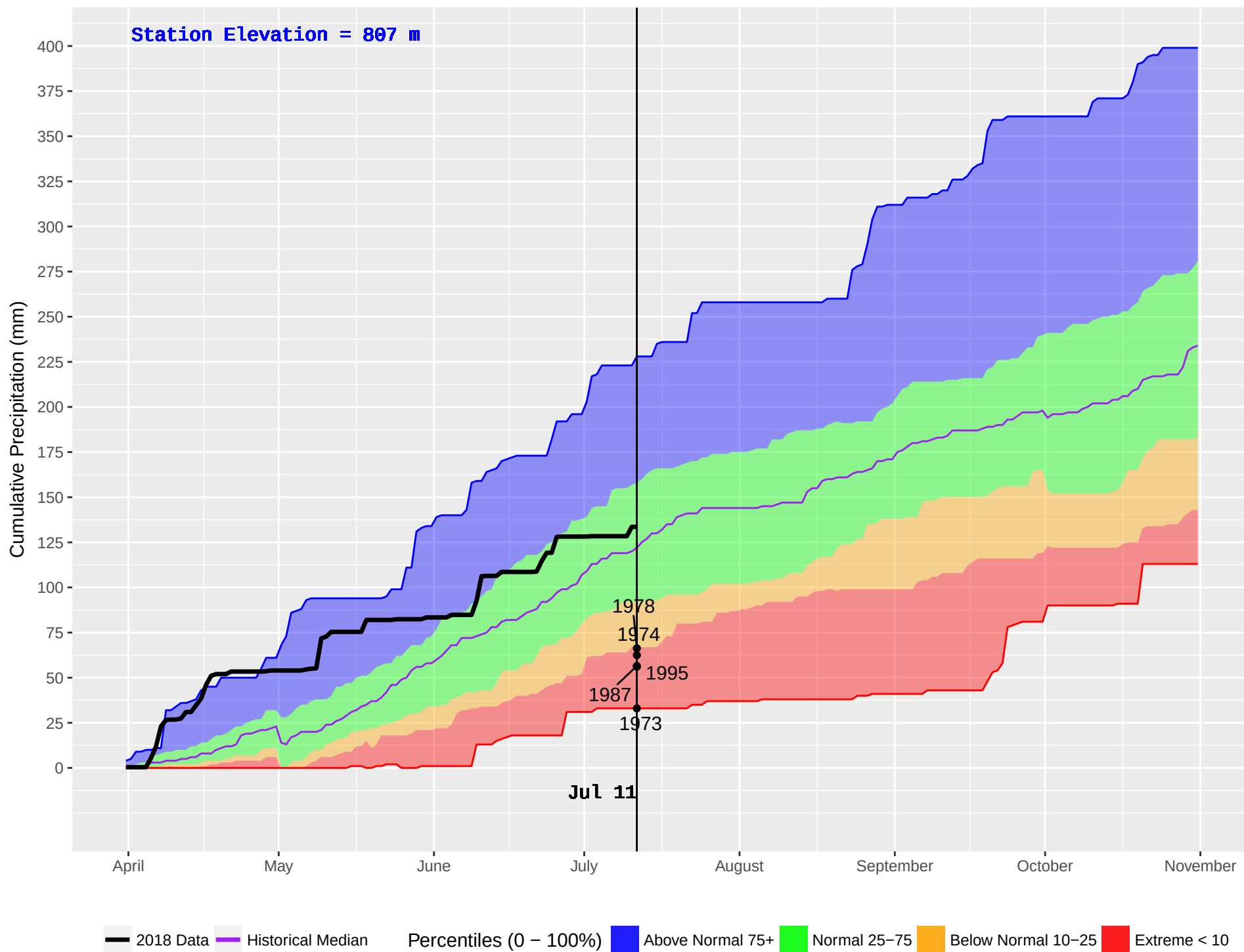
BEAVERDELL (390) : Historical (1970–2016) and Current (2018) Noon Cumulative Precipitation
