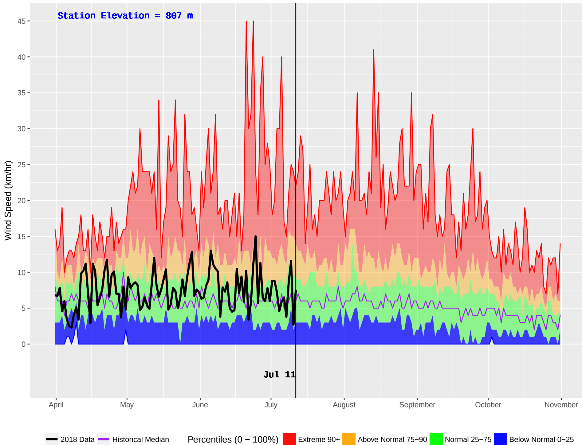
BEAVERDELL (390) : Historical (1970–2016) and Current (2018) Noon Wind Speed
