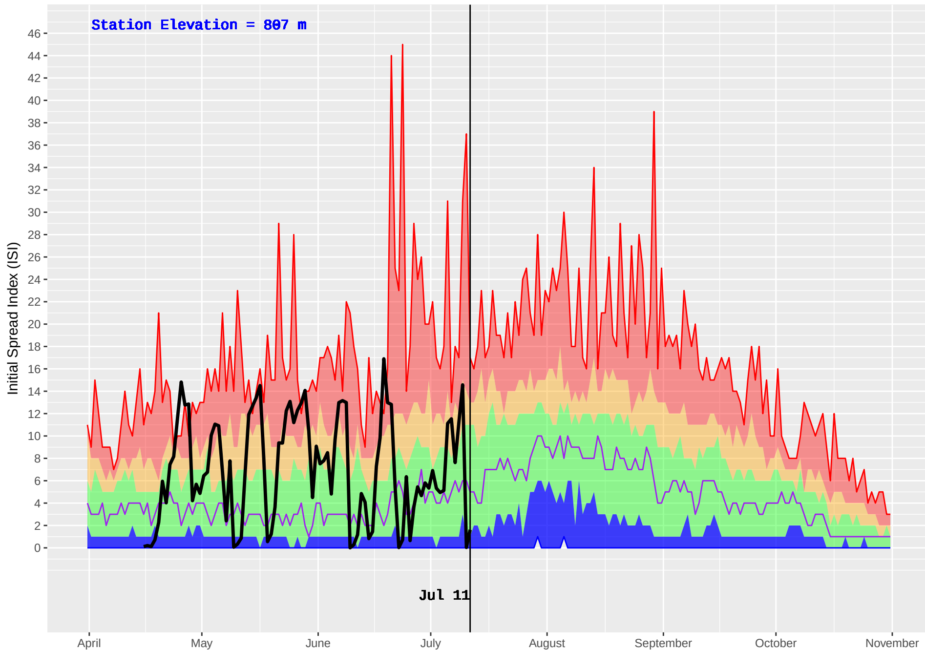
BEAVERDELL (390) : Historical (1970–2016) and Current (2018) Noon Initial Spread Index (ISI)
