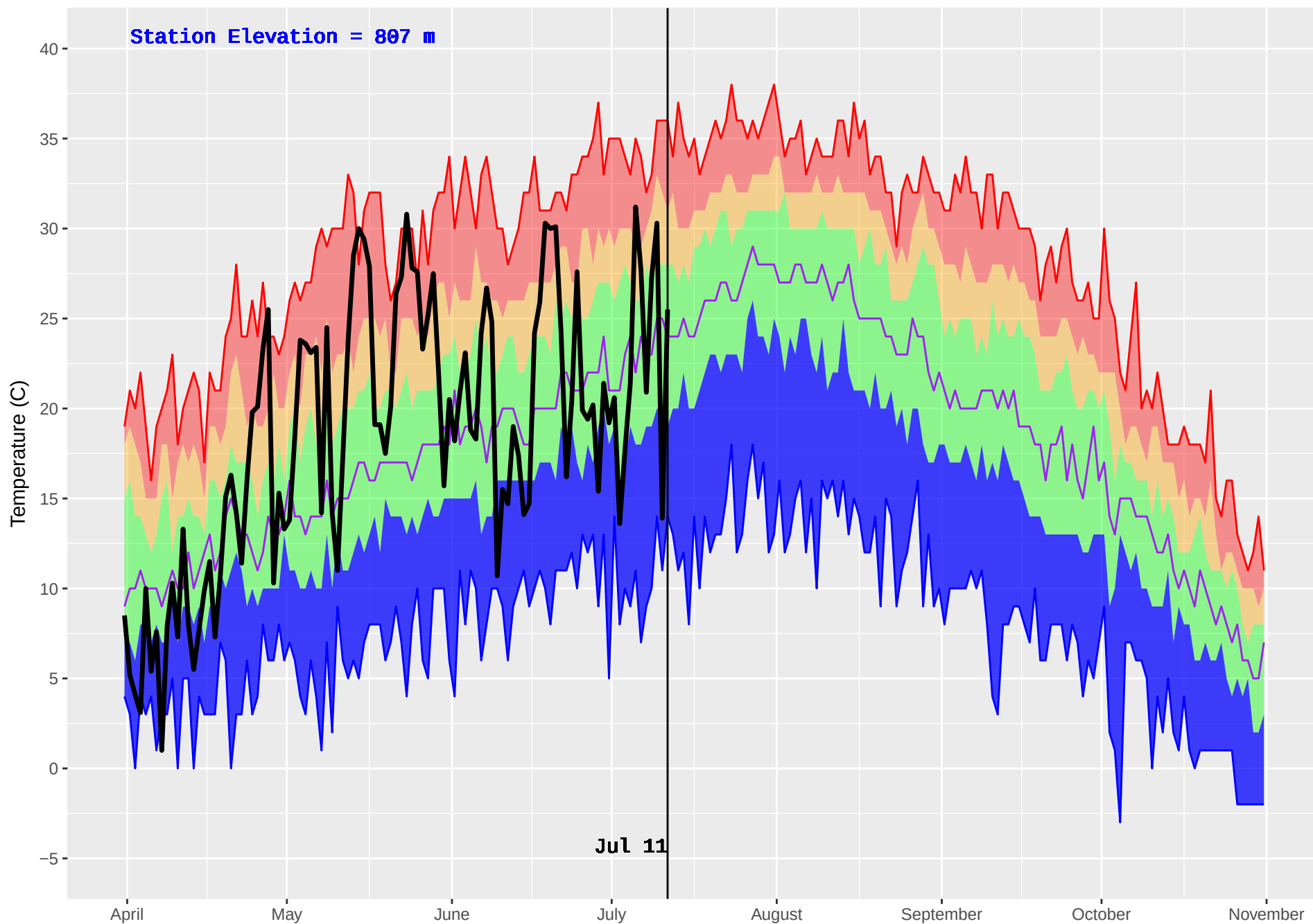
BEAVERDELL (390) : Historical (1970–2016) and Current (2018) Noon Temperature
