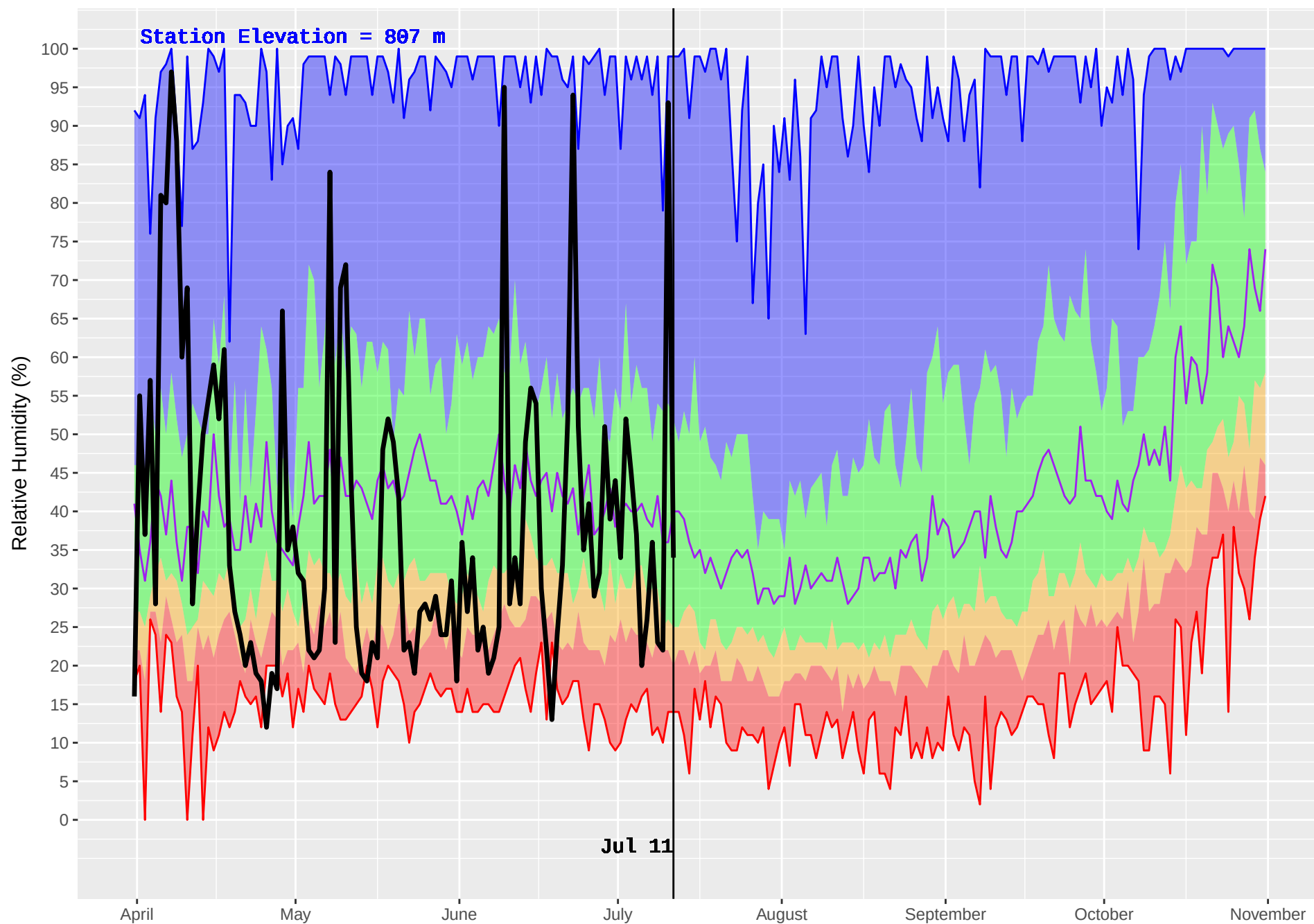
BEAVERDELL (390) : Historical (1970–2016) and Current (2018) Noon Relative Humidity
