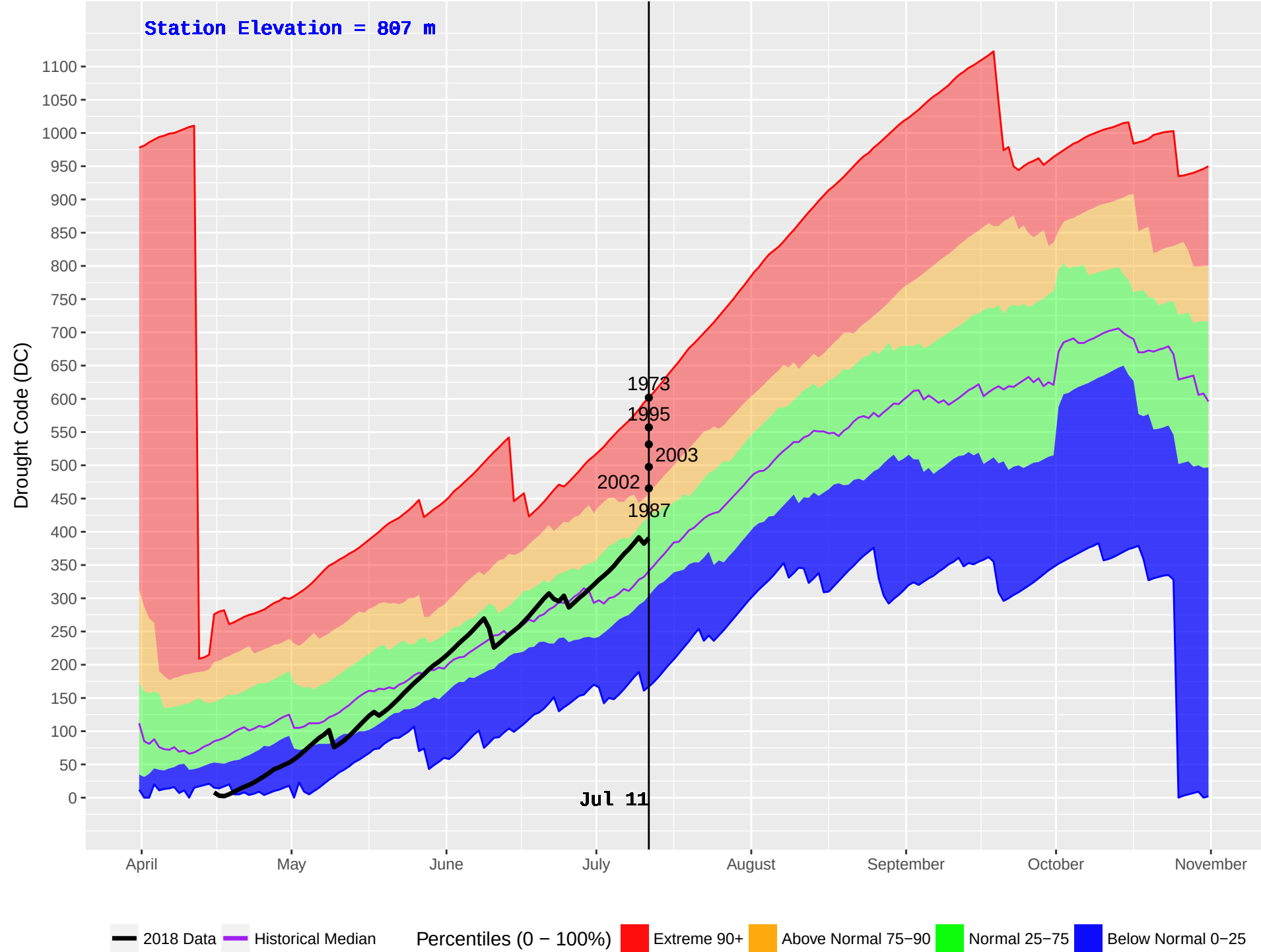
BEAVERDELL (390) : Historical (1970–2016) and Current (2018) Noon Drought Code (DC)
