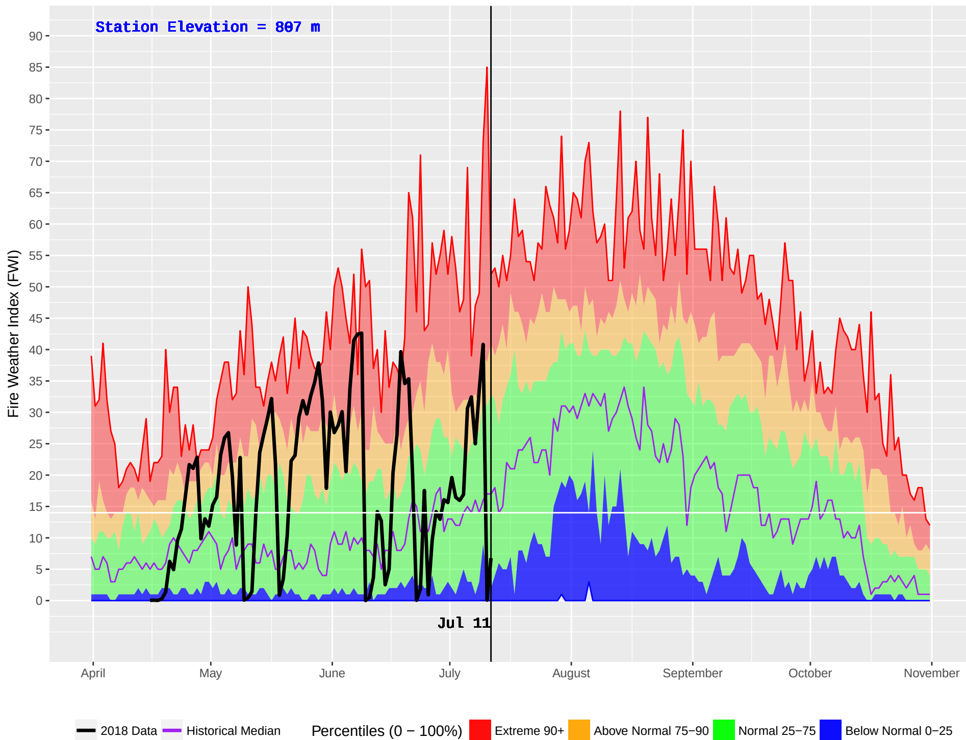
BEAVERDELL (390) : Historical (1970–2016) and Current (2018) Noon Fire Weather Index (FWI)
