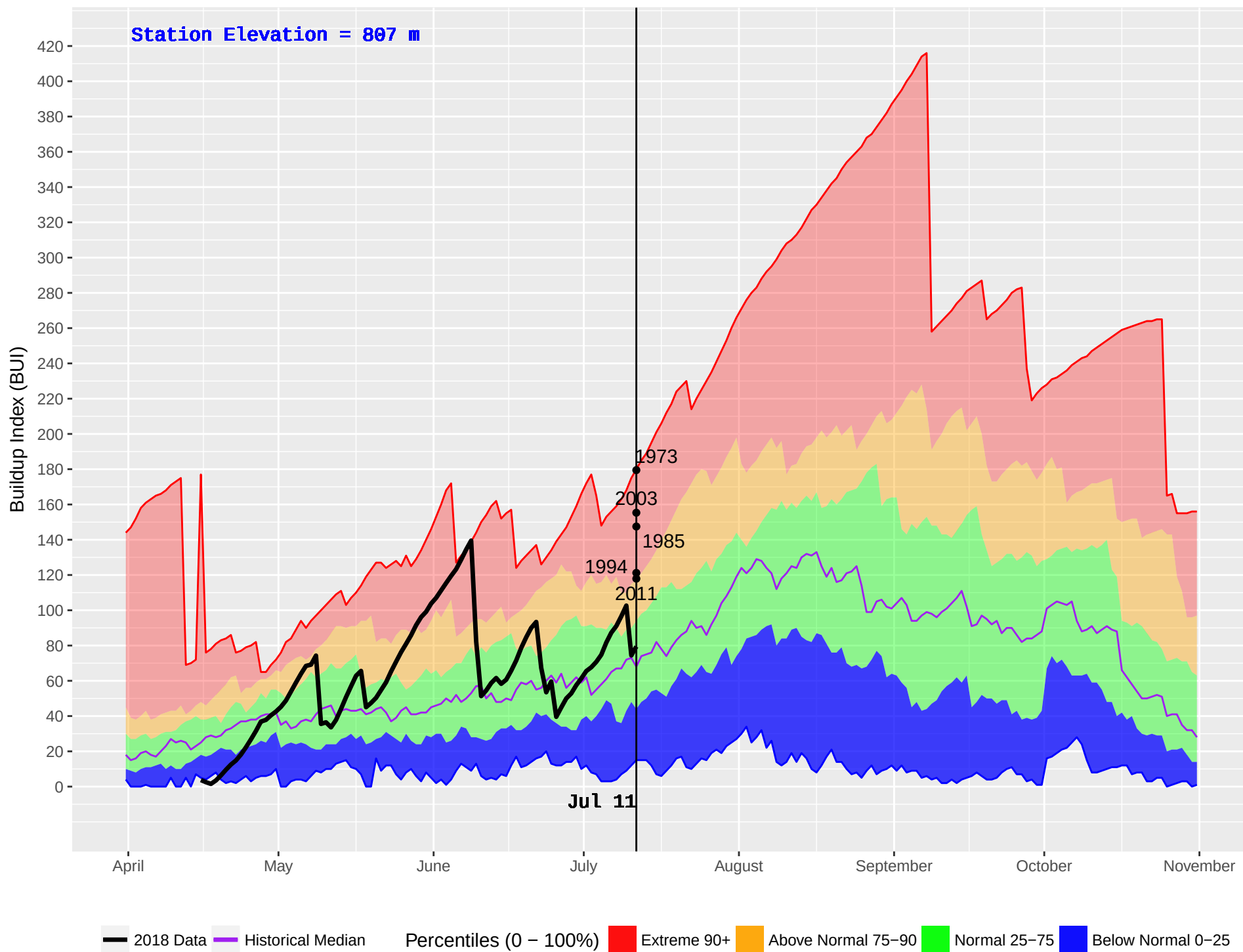
BEAVERDELL (390) : Historical (1970–2016) and Current (2018) Noon Buildup Index (BUI)
